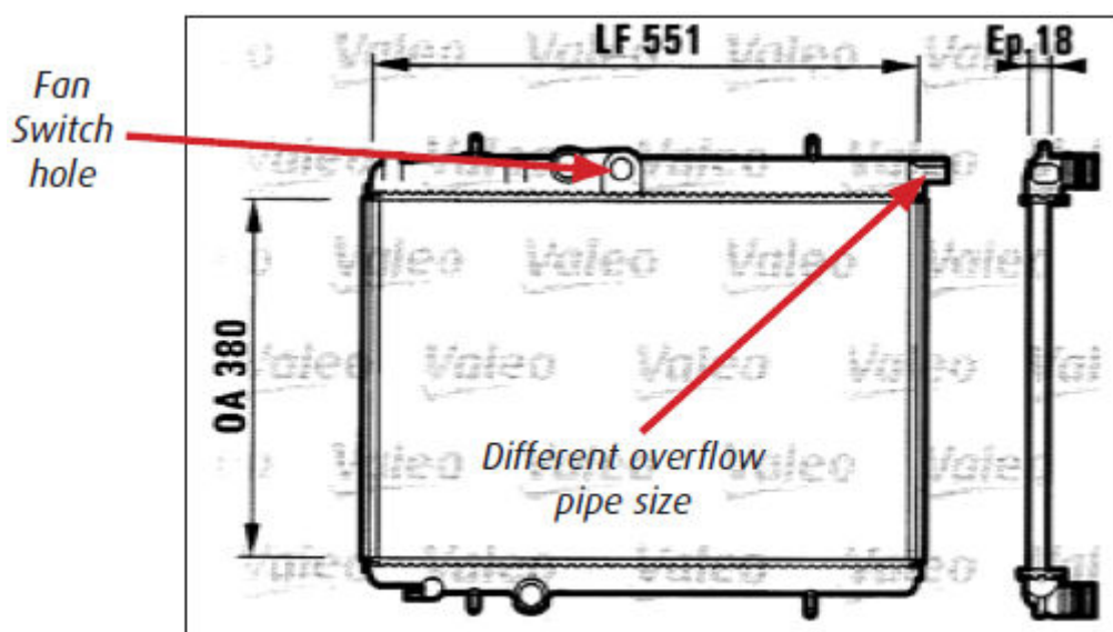
Technical drawing of 732886
